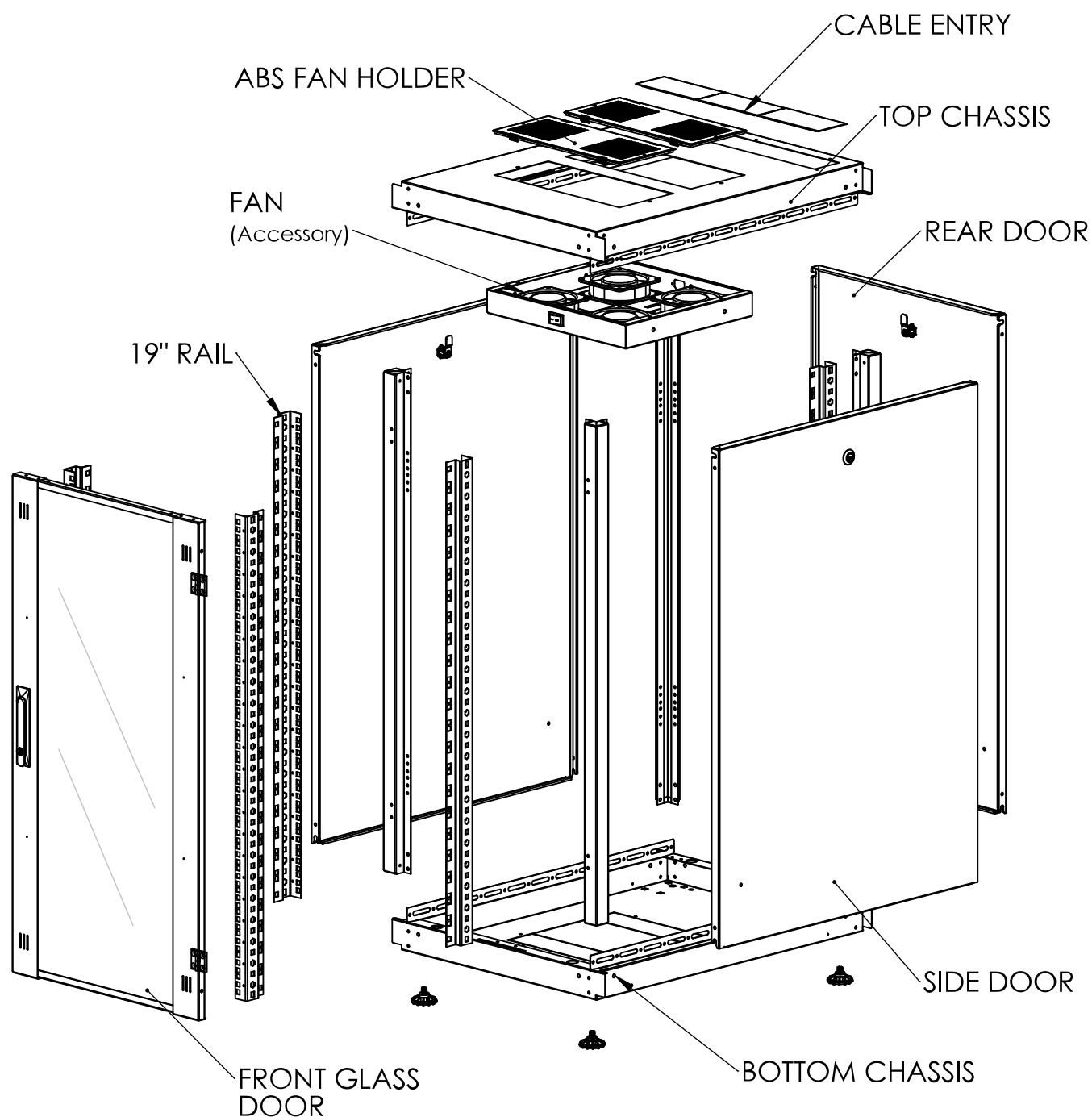
Exploded view
