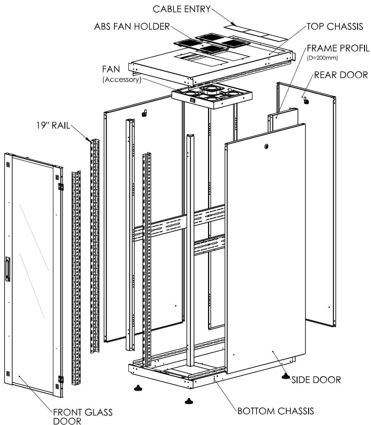
Exploded view
