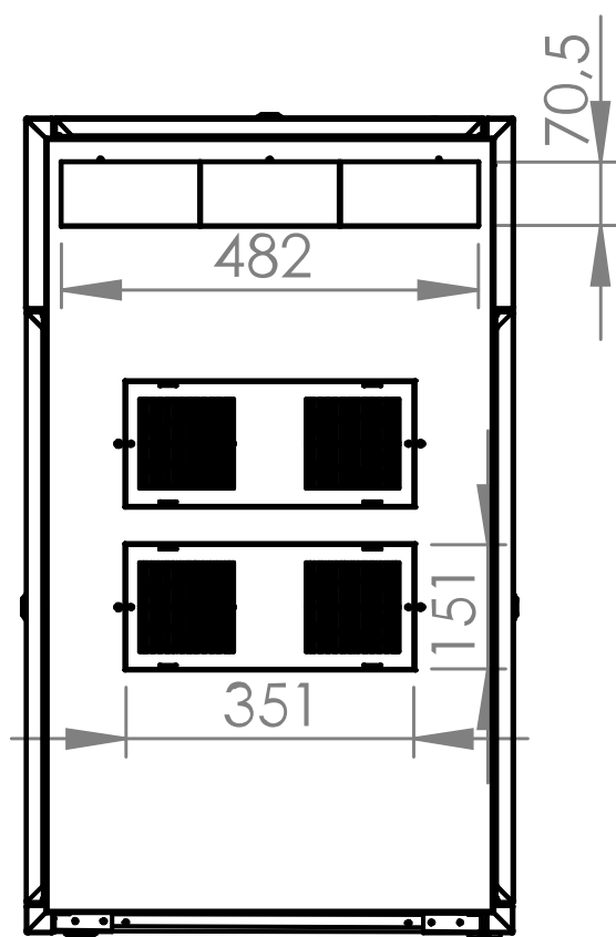
Top view
