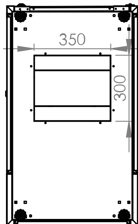
Bottom view
