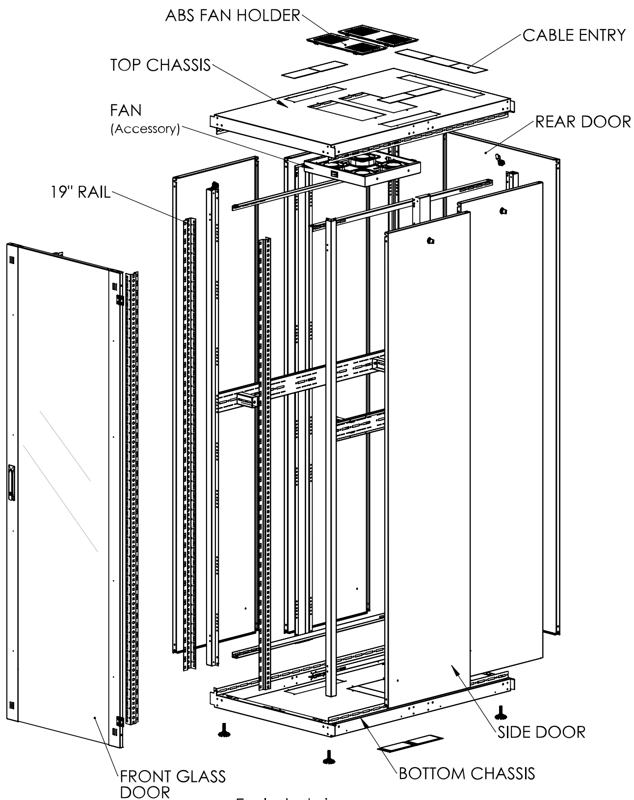
Exploded view
