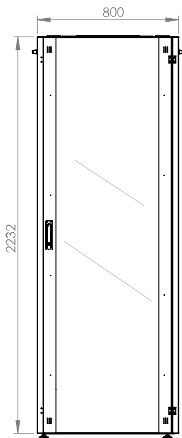
Front view
