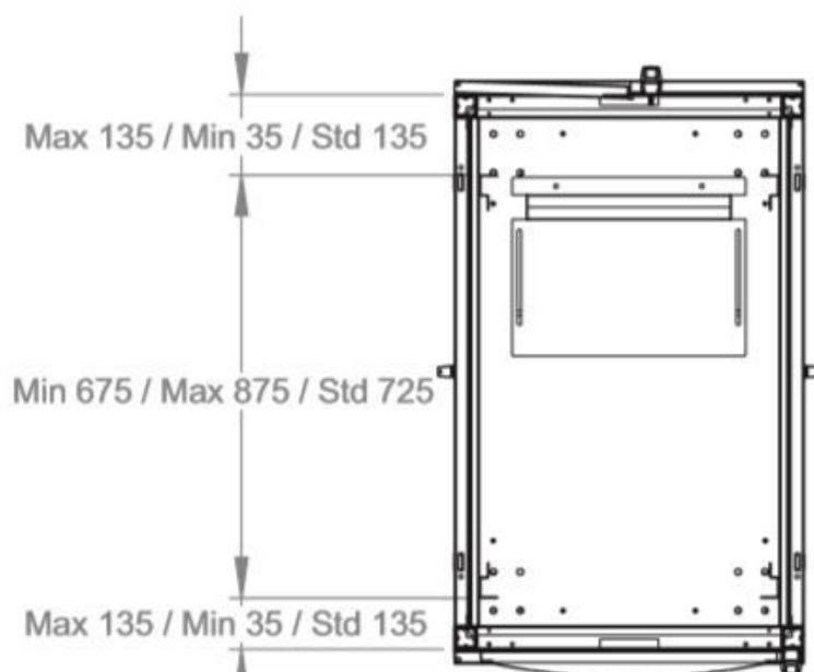
Max/Std/Min Equipment mounting distance
